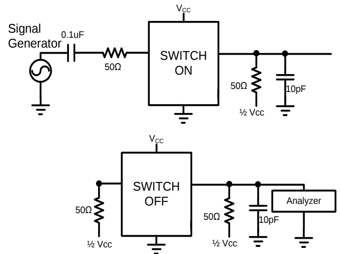
Figure 5 Crosstalk
