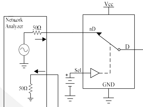
Figure 5 Bandwidth
