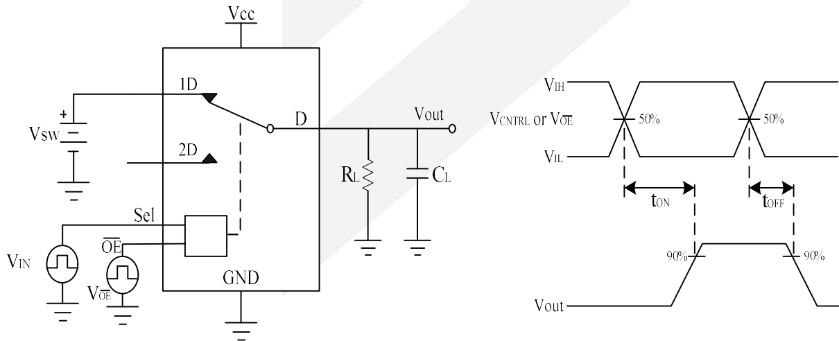
Figure 9 Turn-On/Turn-Off
