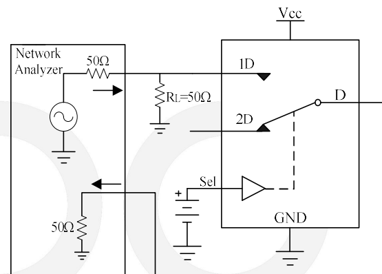
Figure 7 Off-isolation
