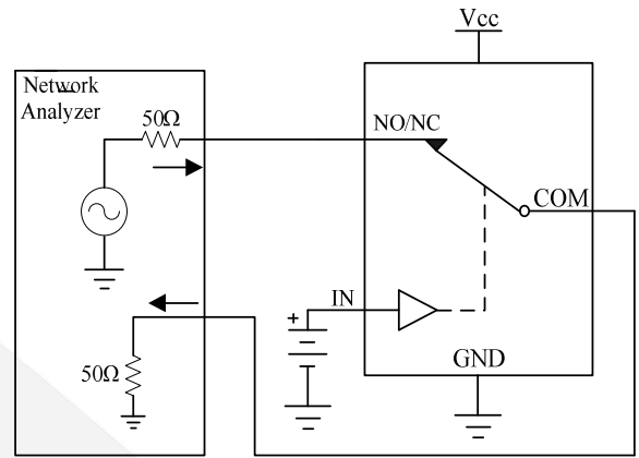
Figure 5 Bandwidth
