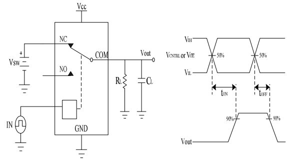
Figure 9 Turn-On/Turn-Off
