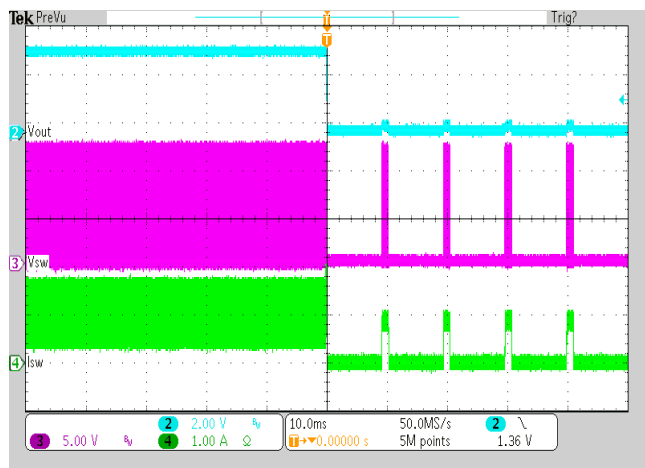
Figure 8 Short Circuit Protection (Vin=12V, Vout=3.3V, Load=1A)
