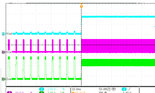
Short Circuit Recovery ( V_{IN}=12V, V_{OUT}=3.3V, Load=3A )
