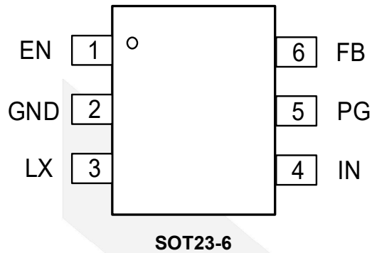
Figure 1 Pin Assignment (Top View)
