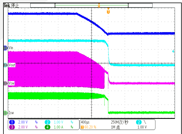
Shut down from VIN ( V_{IN}=5V , V_{OUT}=1.8V , Load=1.2A)
