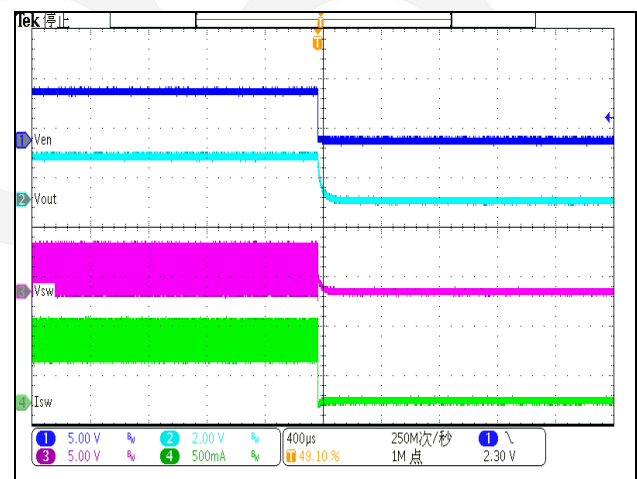
Shut down from Enable ( V_{IN}=5V , V_{OUT}=1.8V , Load=0.6A)
