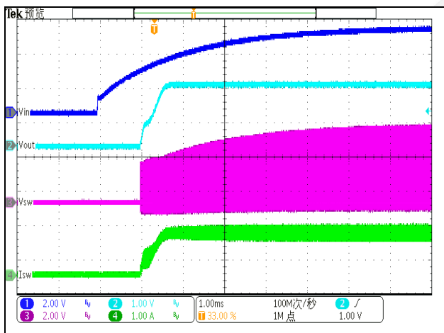
Start up from VIN ( V_{IN}=5V , V_{OUT}=1.8V , Load=1.2A)
