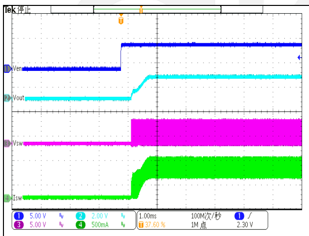
Start up from Enable ( V_{IN}=5V , V_{OUT}=1.8V , Load=0.6A)
