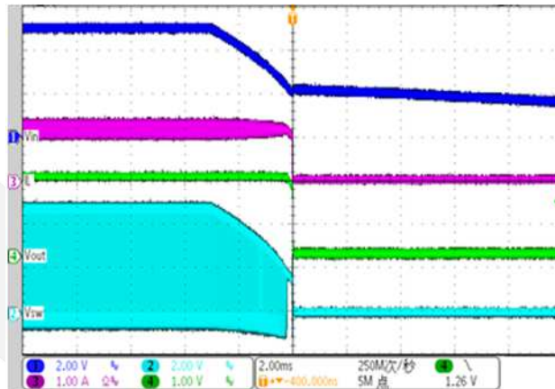
Shutdown from Vin (Iload=1.2A)
