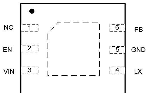
DFN-6
