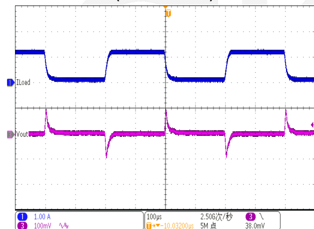
Load transient (Iload=0.1-1.2A)
