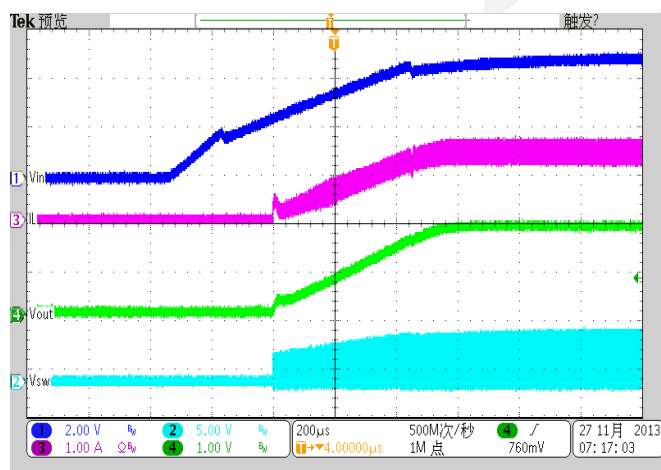
Start up from Enable ( V_{IN}=5V , V_{OUT}=1.8V , Load=1.5A)
