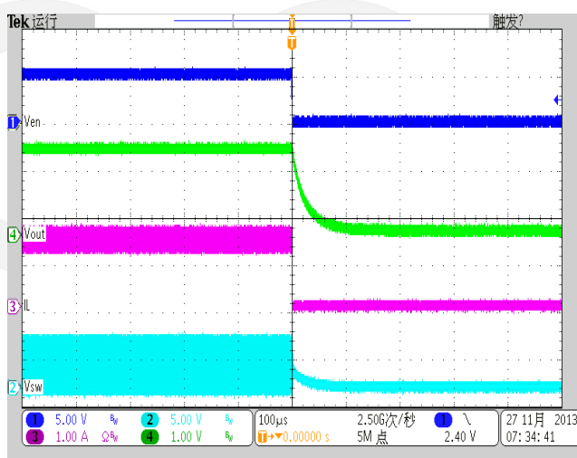
Shut down from Enable ( V_{IN}=5V , V_{OUT}=1.8V , Load=1.5A)
