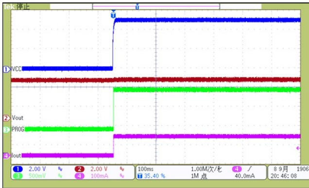
Charging Curve
