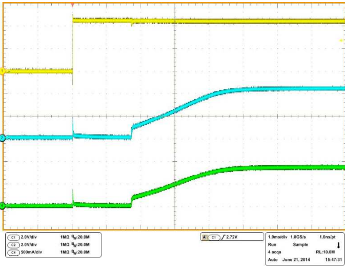
V_{IN}=5V, R_{OUT}=5.1\Omega, V_{IN} Startup
